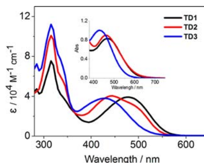
Figure 2. UV-vis absorption spectra of TD1–3 in THF and on \text{TiO}_2 films (inset).
